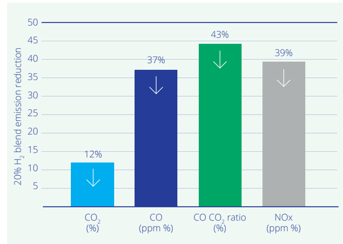
Figure 8. Average percentage reduction in emissions measured for the boilers tested with 20% hydrogen blend.
